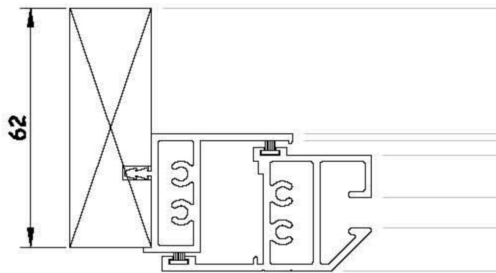
Hinged Unit Jamb detail.
