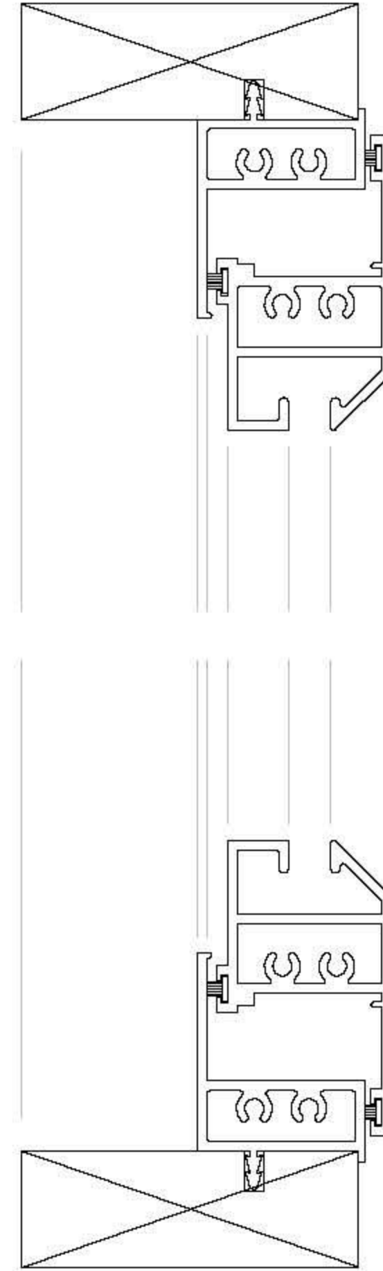
Section through the Hinged Unit frame.
