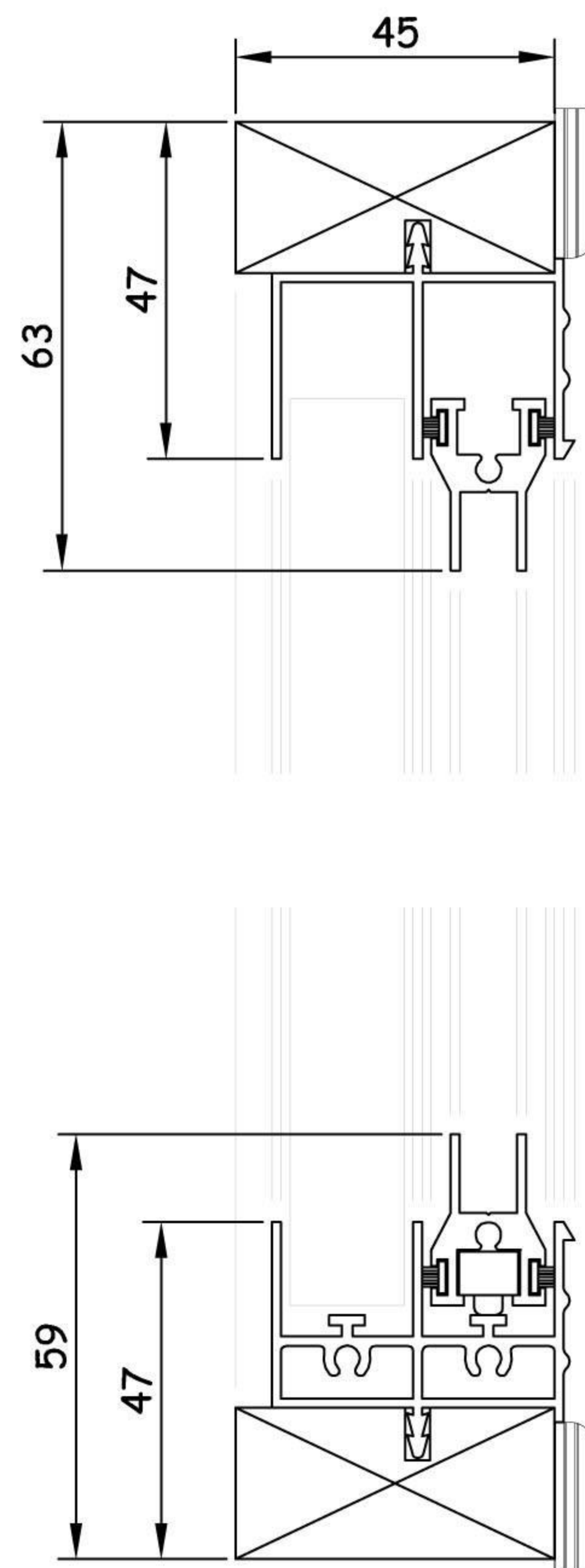
Section through the Horizontal Slider.
