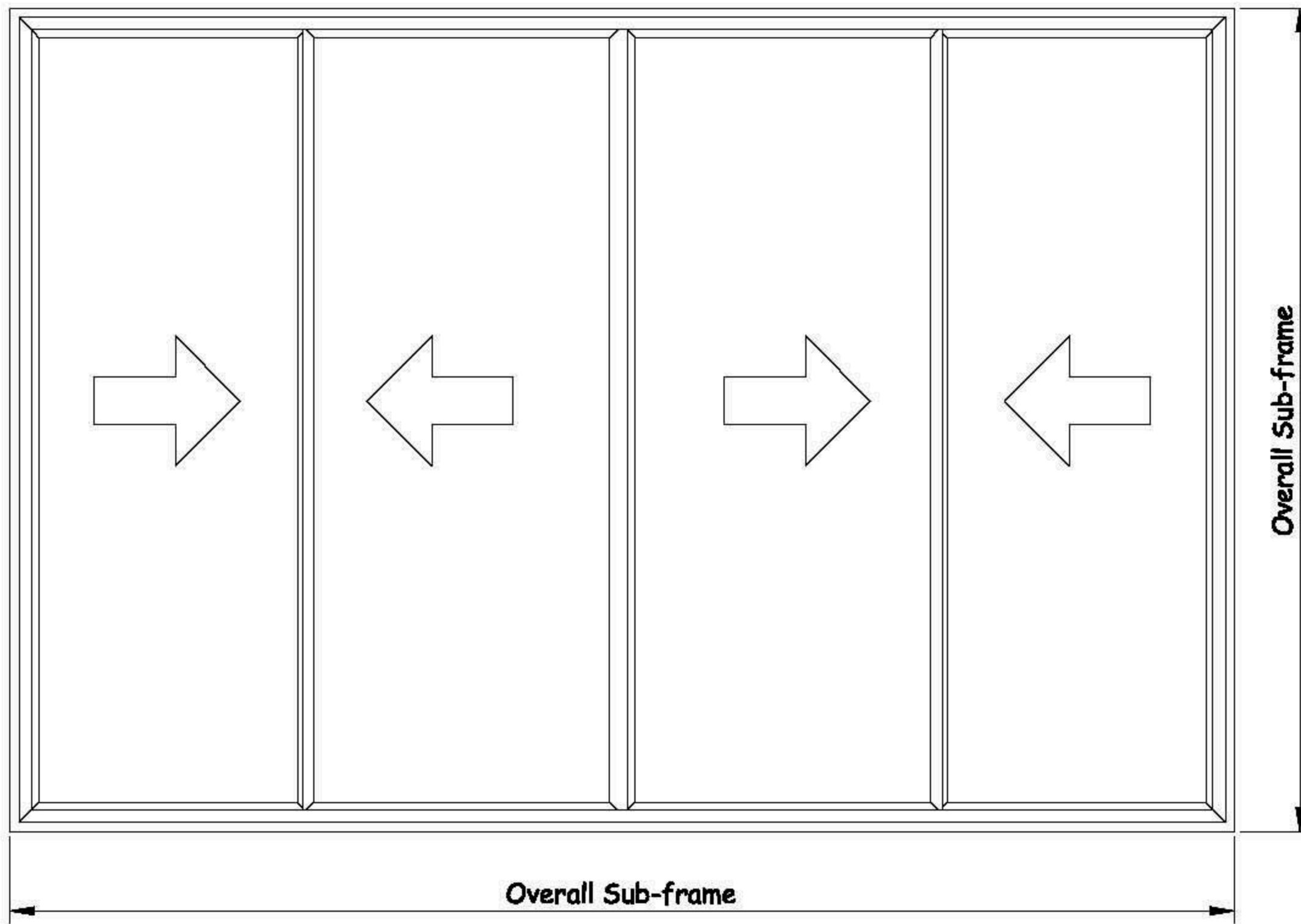
Typical elevation of an SS4 Horizontal Slider.
