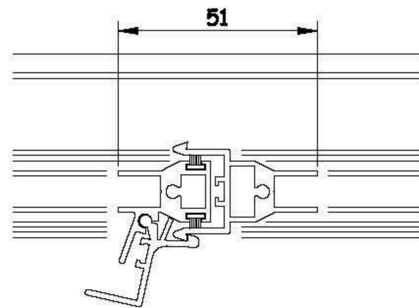
Centre interlocker detail.
